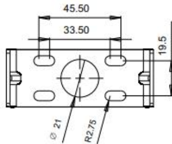
Bracket Dimensions
