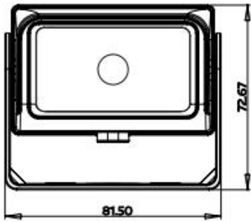
Bracket Dimensions
